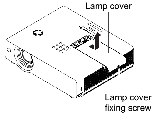
Lamp unit fixing screws
