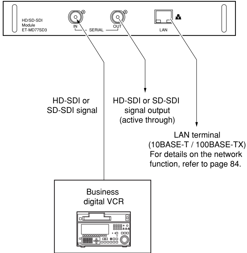
HD/SD-SDI input module (optional) ET-MD77SD3 (for HD/SD)
