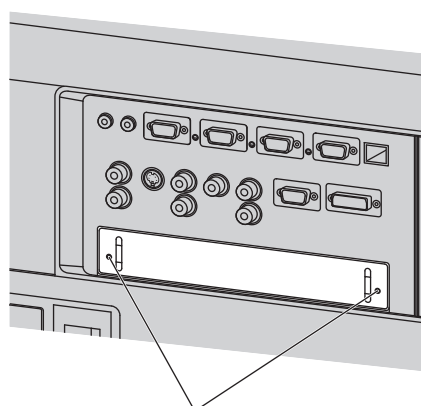
Remove 2 screws.
