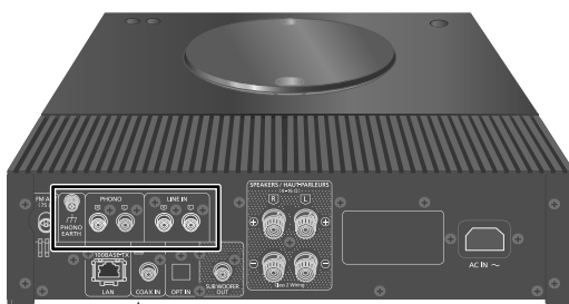
Analog audio output device (Turntable, Blu-ray Disc player, etc.)
